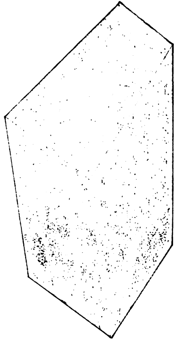
Fig. 18.—Type of Hornbeam-wood ( Carpinus ).
